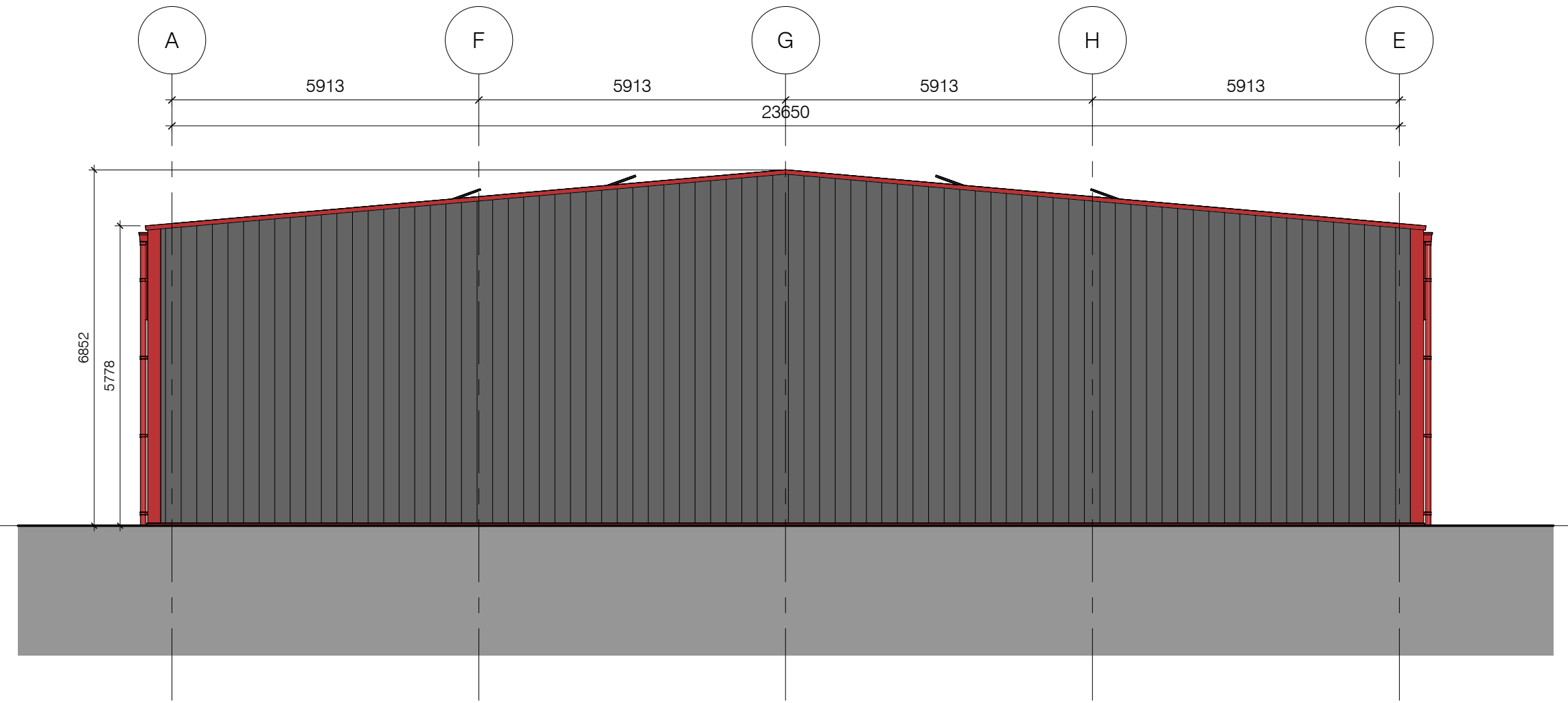
North Elevation (side) 1:100
