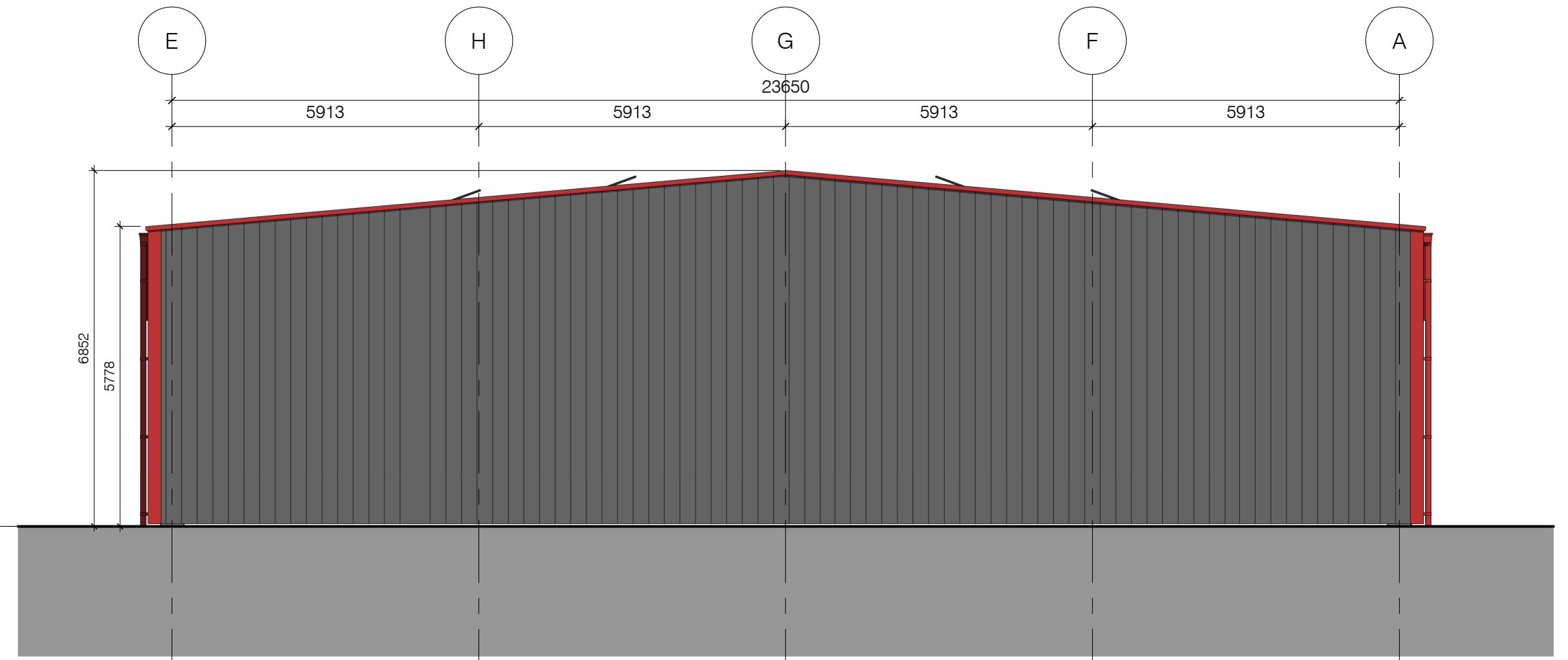
South Elevation (side) 1:100
